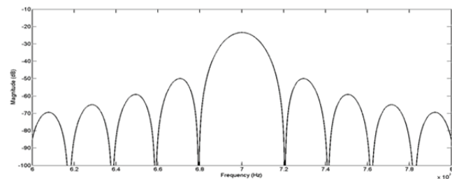
Fig. 4. Simulated response of the same device, based on the available information.
